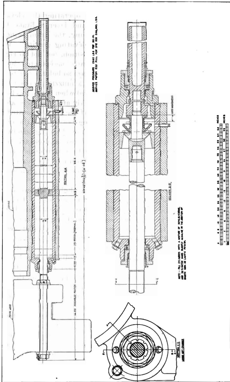
RECOIL, CYLINDER ASSEMBLY (LONG.) 14-INCH RAILWAY MOUNT.
