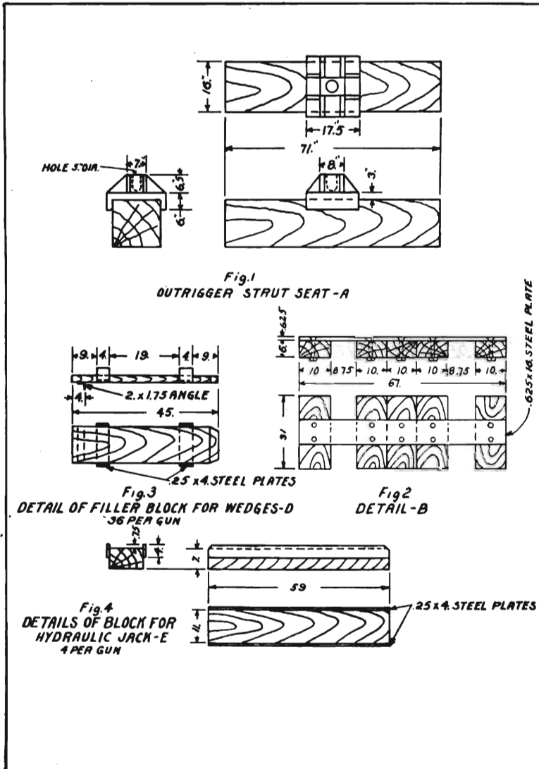
OUTRIGGER FLOAT DETAILS OF 240-MM. GUN, MODEL 1893-1896. 452-22-5
