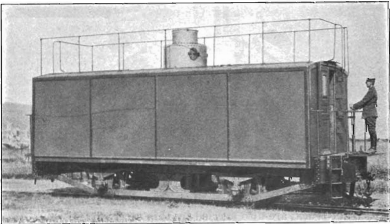
THIS CAR, ALSO A UNIT OF THE 200-MM. HOWITZER TRAIN, IS A COMBINATION PERSONNEL CAR AND OBSERVATORY.
