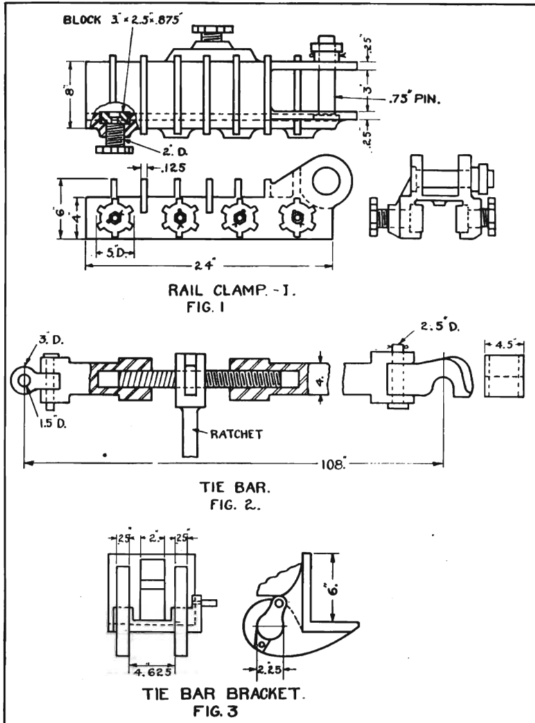
DETAIL SKETCHES OF RAIL CLAMP.
