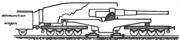
DUE TO CRADLE RECOIL SYSTEM THE "SLIDE" OF MOUNT IS SO REDUCED TO PERMIT COUPLING TO AMMUNITION CAR DURING ACTION.
