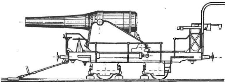
240-MM. HOWITZER MODEL OF 1876 ON TWO AXLE CAR.
