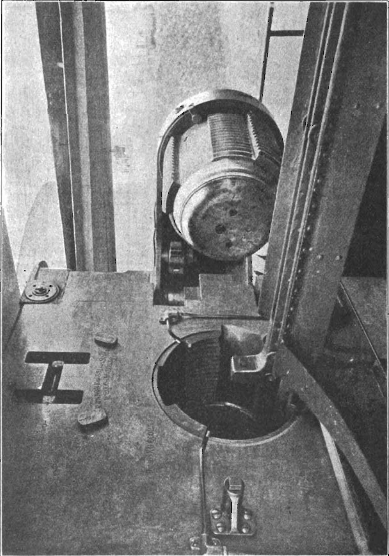
BREECH END OF GUN WITH CHAIN RAMMER ENTERING SCREW BOX.
