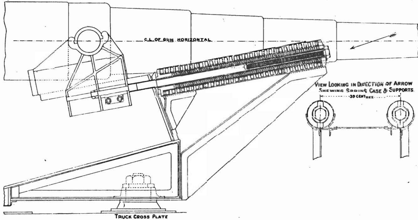
TRUCK CROSS PLATE COUNTER-RECOIL MECHANISM 9.2-INCH GUN (PARA. 226).
