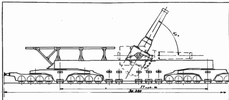
RAILWAY MOUNT OF SLIDING TYPE MOUNTING 520-MM. HOWITZER WITH CRADLE RECOIL.
