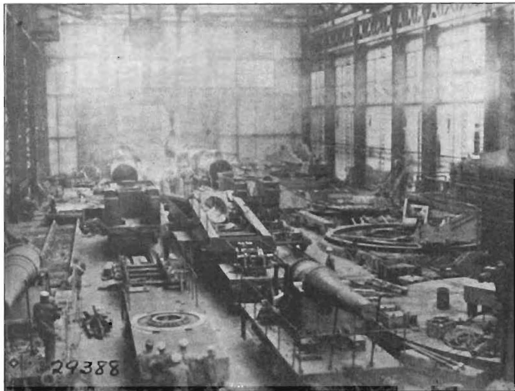
16-INCH, 50-CALIBER AMERICAN NAVY GUN MOUNT, MARK I, IN COURSE OF ERECTION IN THE CHANTIERS DE LA LOIRE ST. NAZAIRE, FRANCE.
