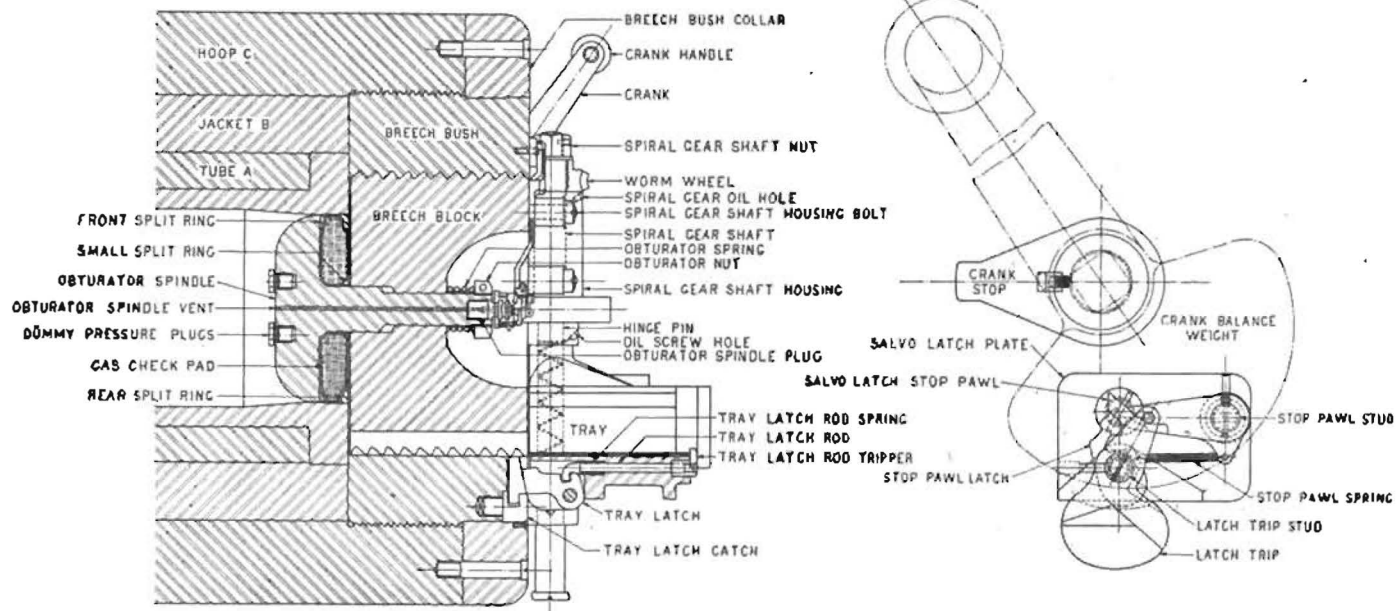
12 INCH GUN MODEL OF 1918 (BETHLEHEM) BREECH MECHANISM
