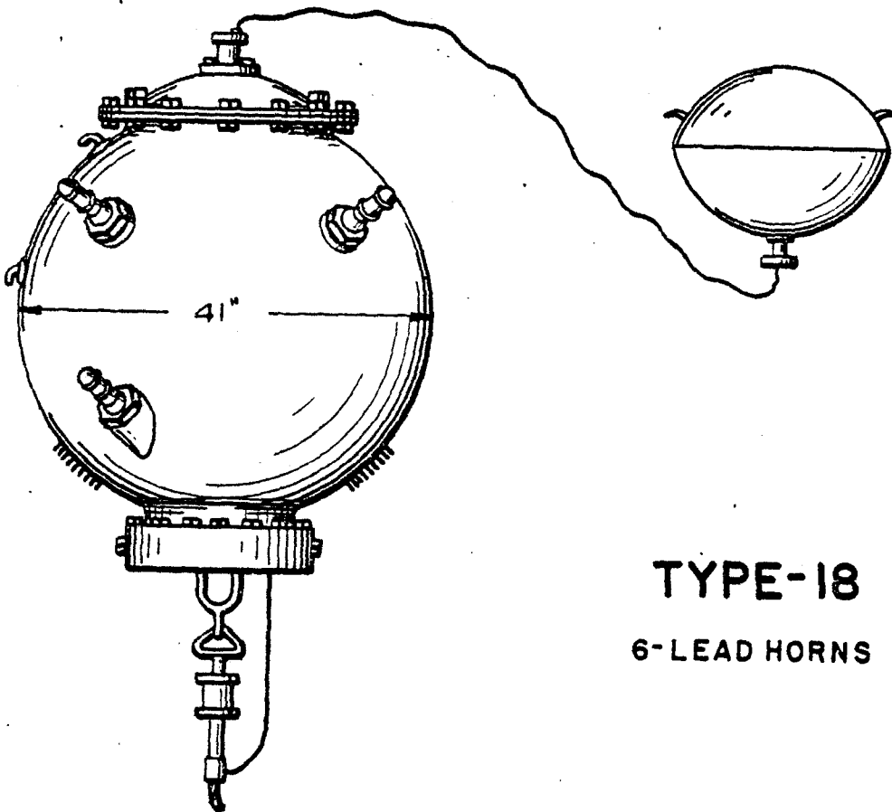
SIDE VIEW
