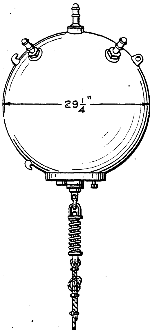
SIDE VIEW
