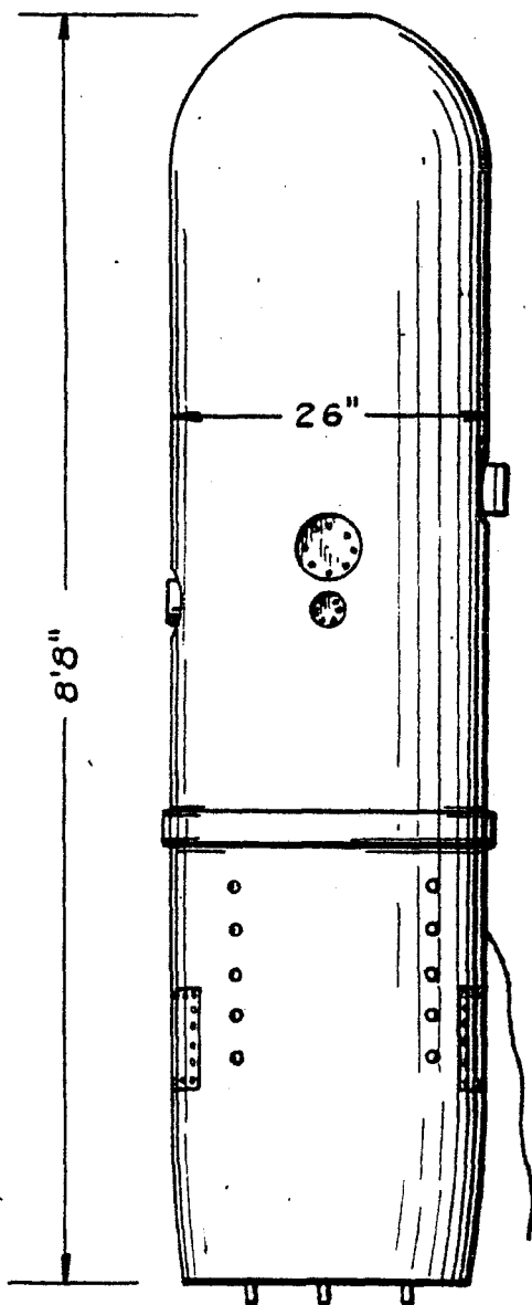
SIDE VIEW
