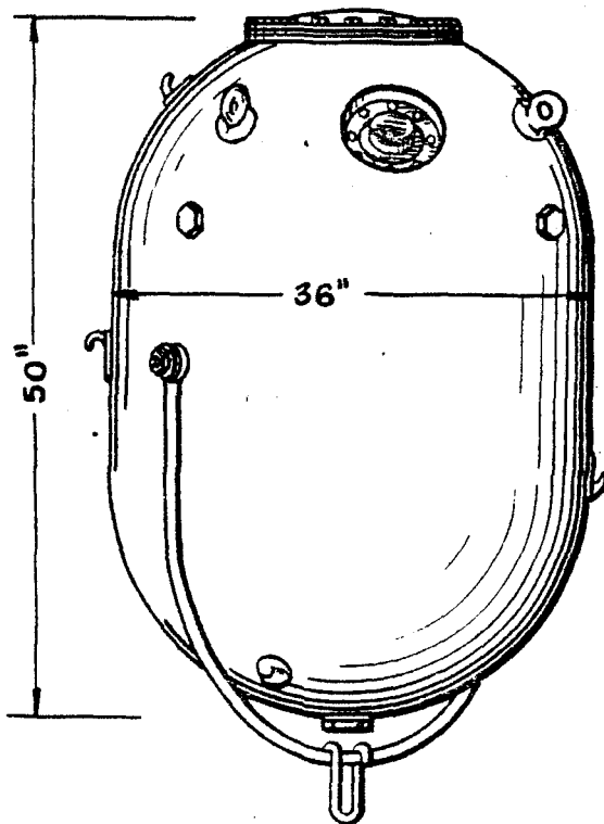
SIDE VIEW
