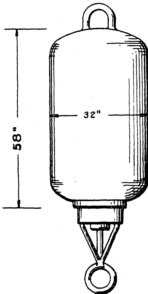
SIDE VIEW
