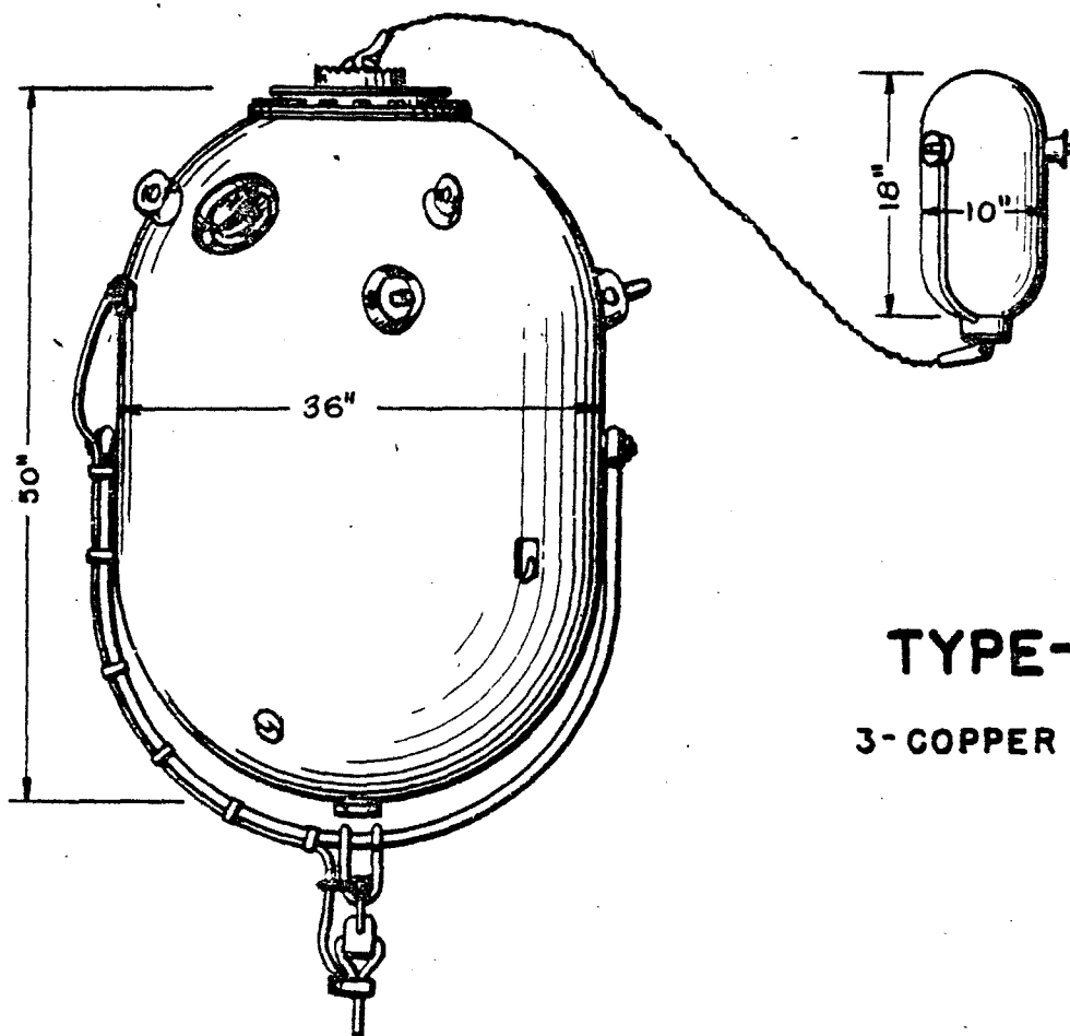
SIDE VIEW
