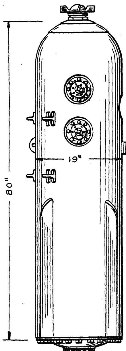
SIDE VIEW
