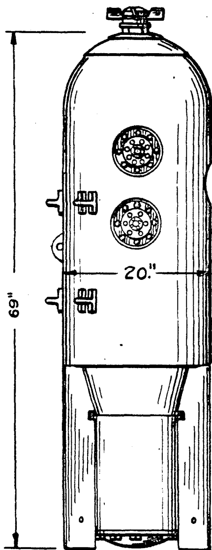
SIDE VIEW
