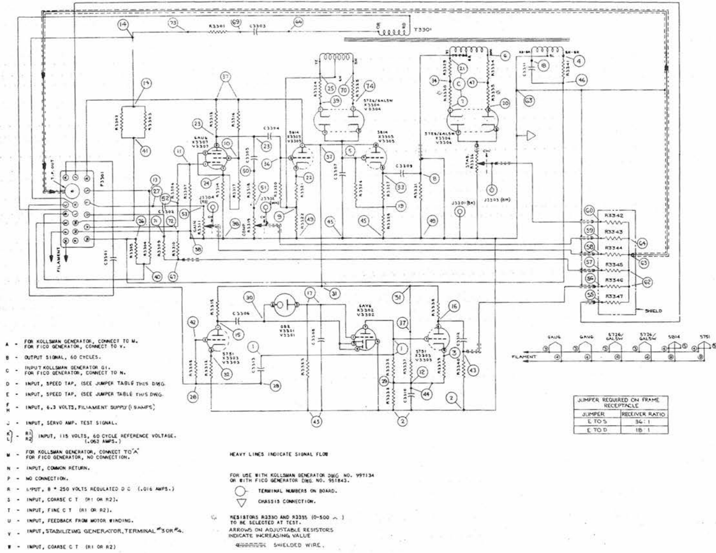
Figure 81. Servo Control, Double-Speed, Schematic Diagram (Unit 3305)
