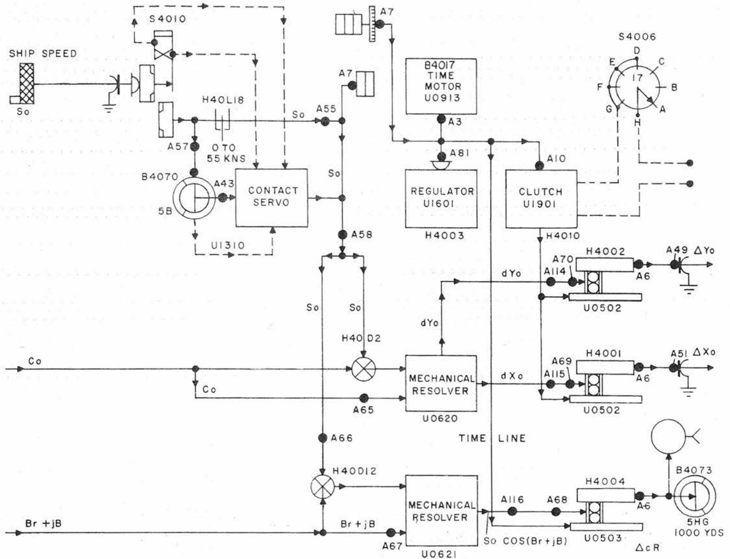
Figure 47. \Delta cR , \Delta Y_o , and \Delta X_o Group
