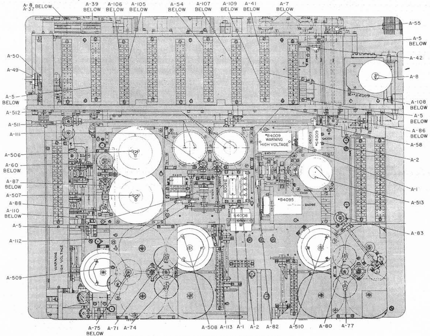
Figure 90. Right Mechanical Section Under Cover No. 6
