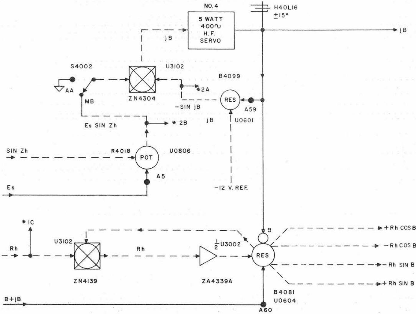
Figure 49. jB Loop and B Resolver
