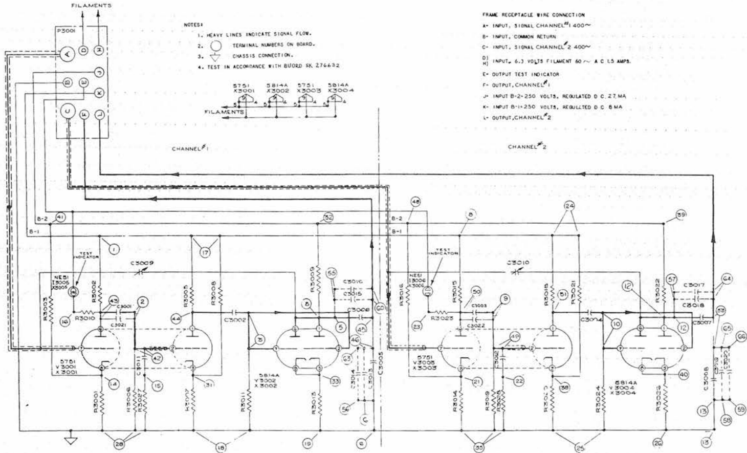
Figure 76. Dual-Channel Amplifier, Schematic Diagram (Unit 3002)
