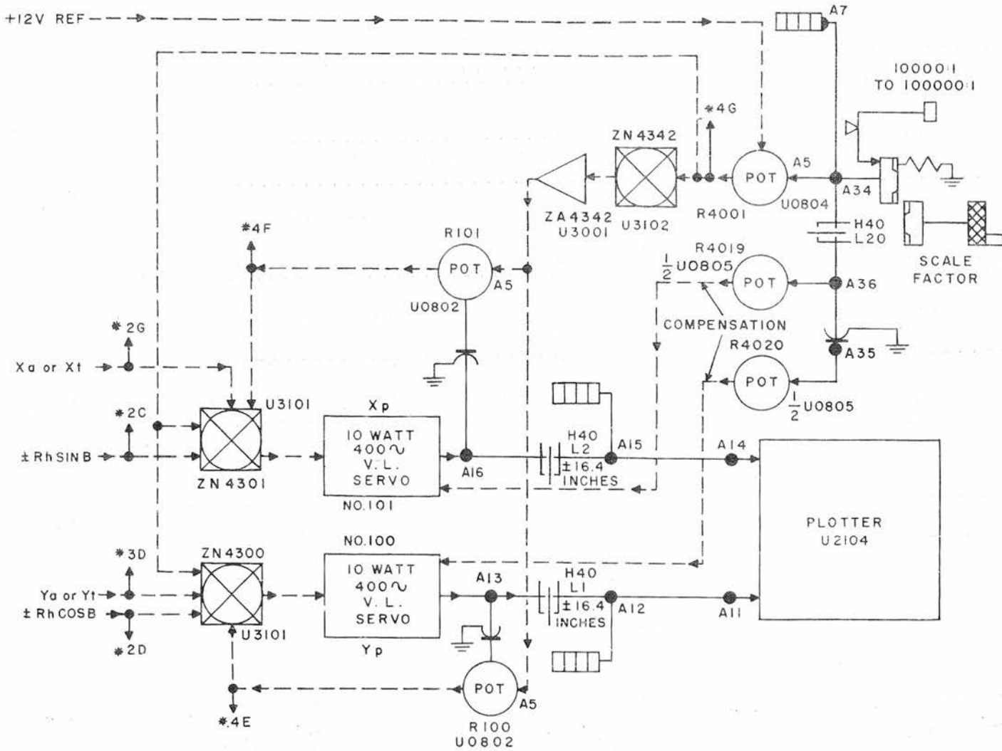
Figure 51. Plotter Group
