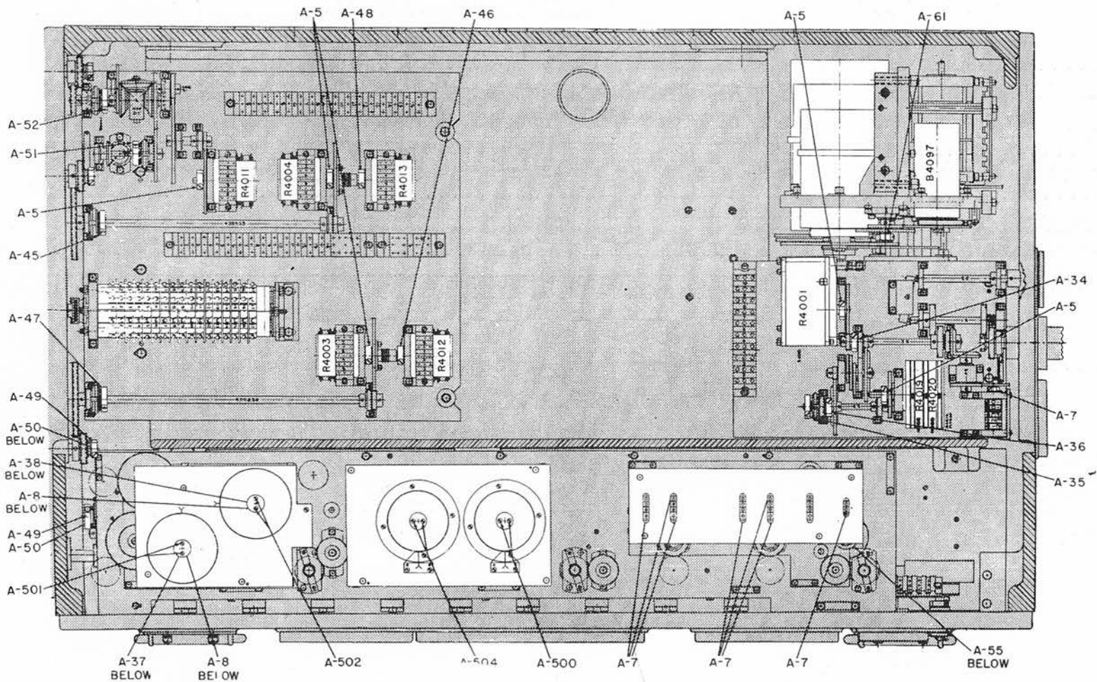
Figure 95. Top Mechanical Section Below Plotter and Cover No. 3
